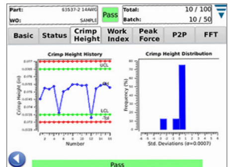
Production Crimp Height
